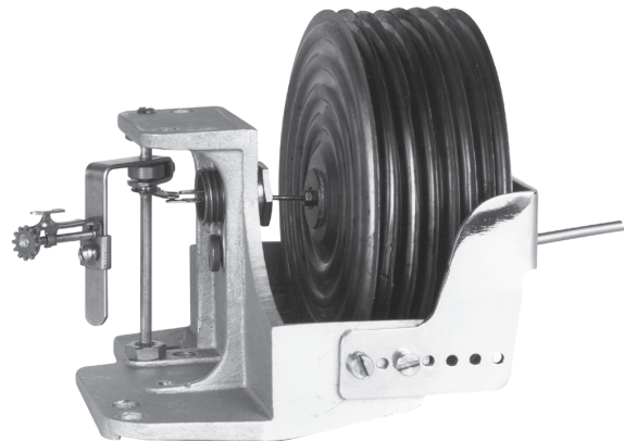
Figure 3. Diaphragm Element
