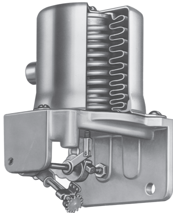
Figure 1. Bellows Element
