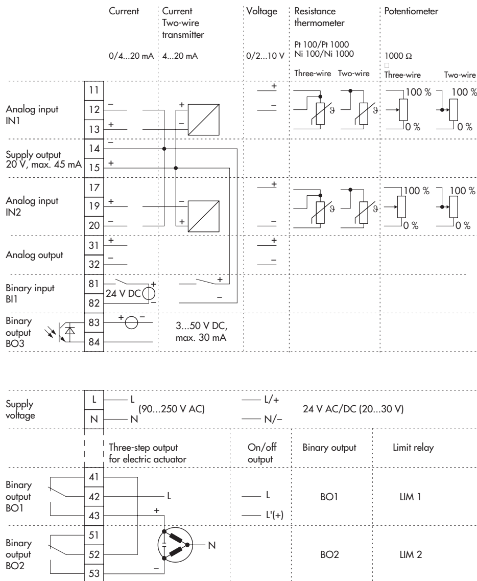
Fig. 6: Electrical connection
