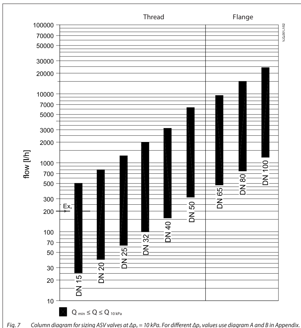
Fig. 7 Column diagram for sizing ASV valves at \Delta p_v = 10 kPa. For different \Delta p_v values use diagram A and B in Appendix.
