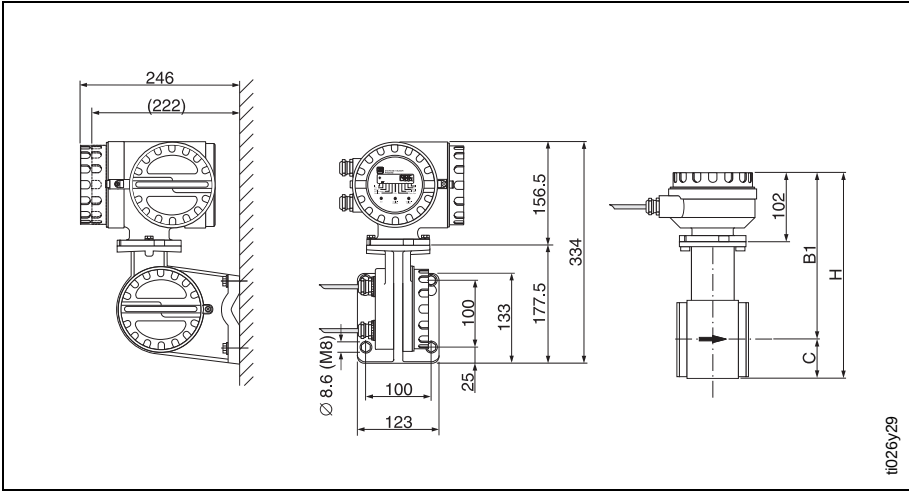
Remote version (FS and FL version)
