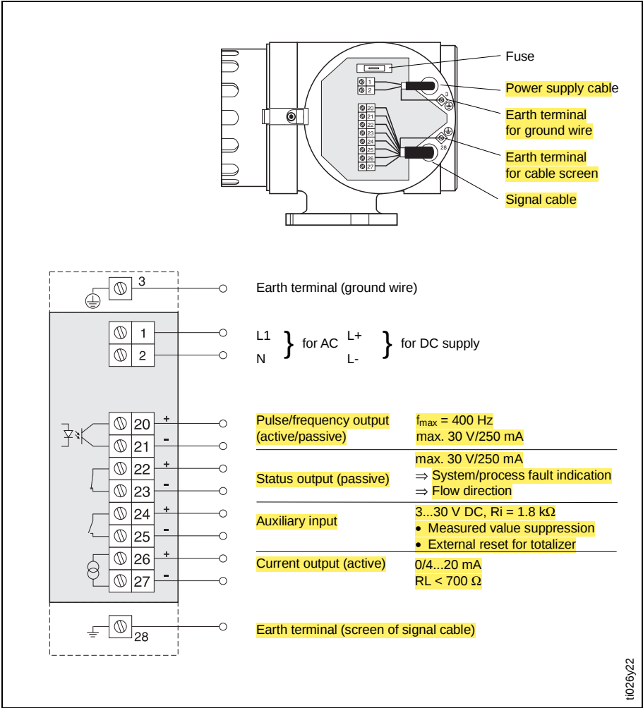
Electrical connection of power supply, input and outputs
