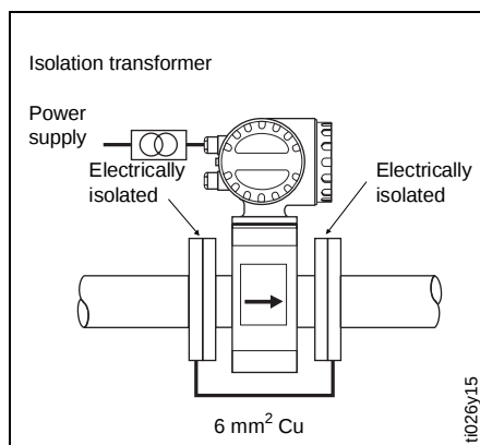
Potential equalisation in lined pipelines with cathodic protection
