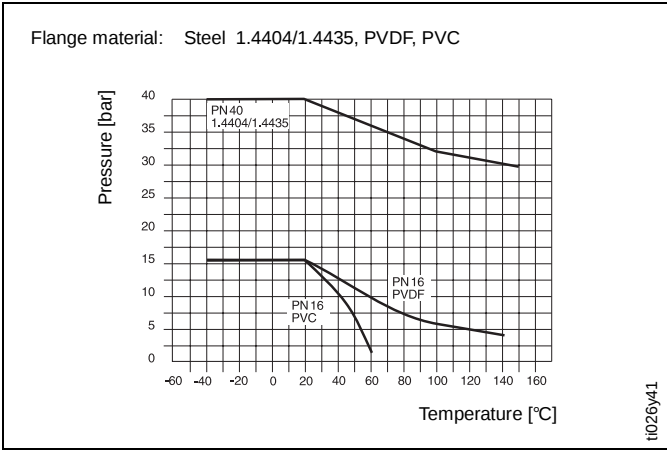
Promag F (DIN 2413 and 2505)
