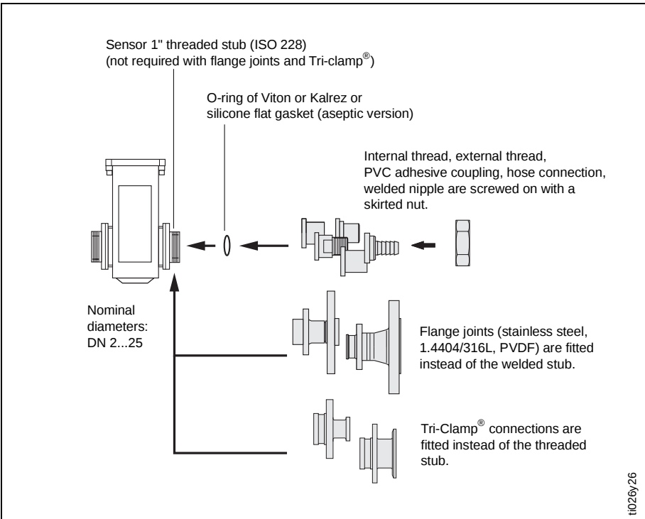
Process connections Promag A
